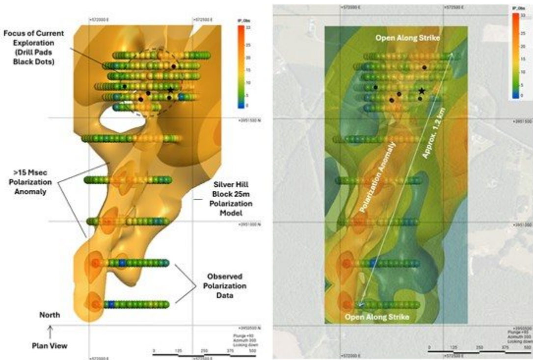
Figure 2: Trended numerical model showing the interpreted connection between raw IP data sets using geologic data including mineralization trends.
