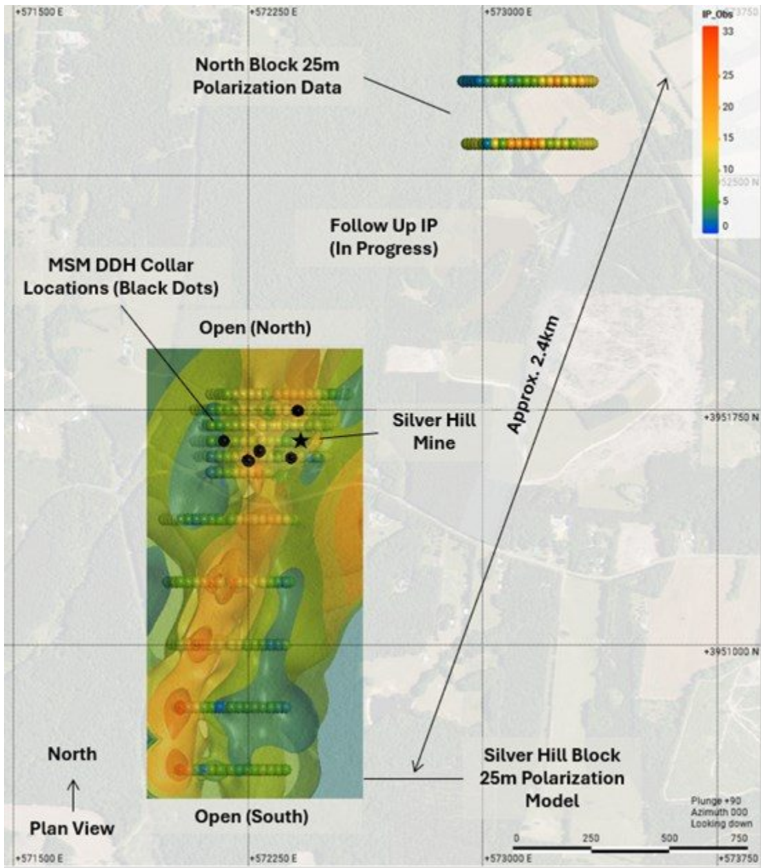
Figure 1: Plan view of 25m PLDP Data showing numerical modeling of induced polarization anomalies relative to current drilling footprint (black dots = MSM diamond drill hole collars).
